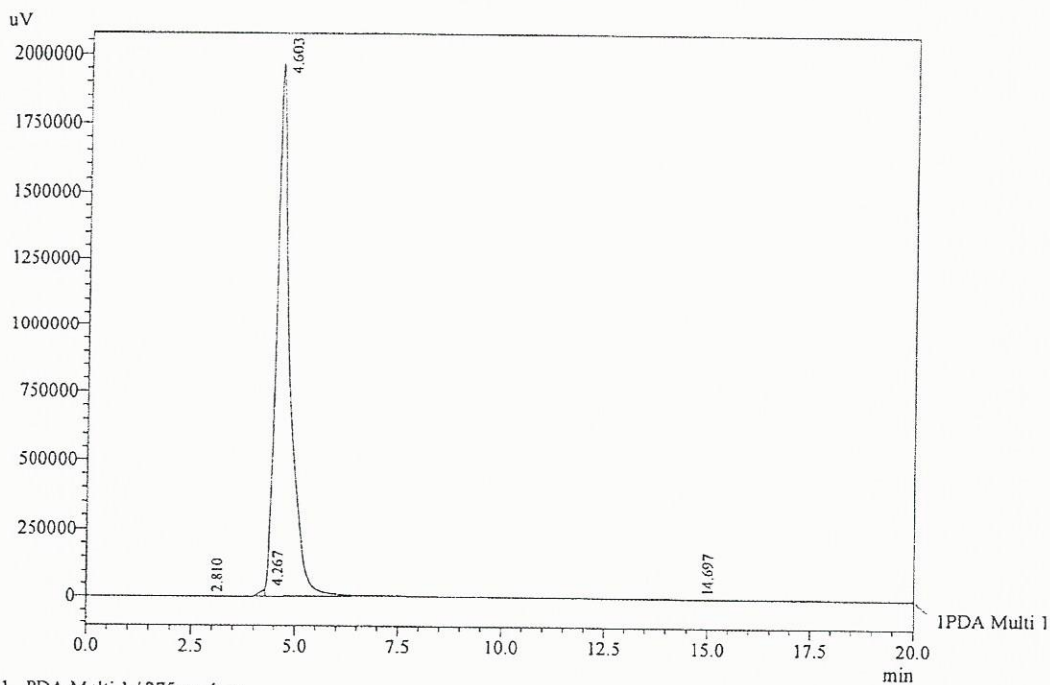
Chromatogram
